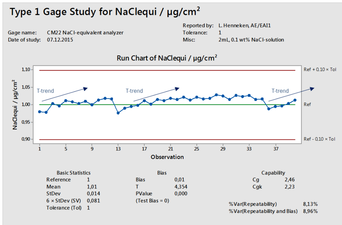
Fig. 4: Analysis of repeatability of \text{NaCl}_{\text{eq.}} / \mu\text{g}/\text{cm} based on 40 measurements of 0.1 wt.-% sodium chloride solution at one site.
